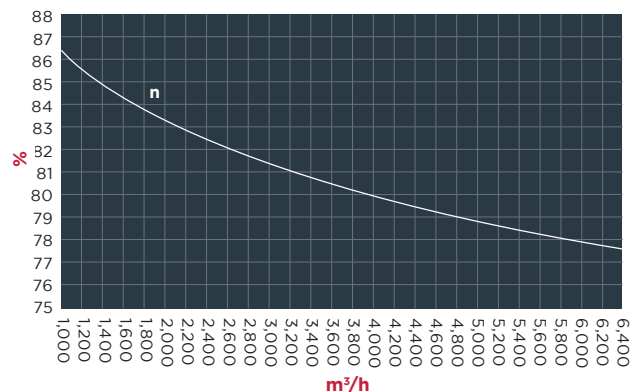
HEAT RECOVERY EFFICIENCY - DIN EN13053 EUROVENT CERTIFIED
