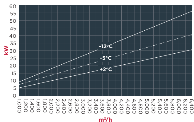
HEAT RECOVERY OUTPUT
